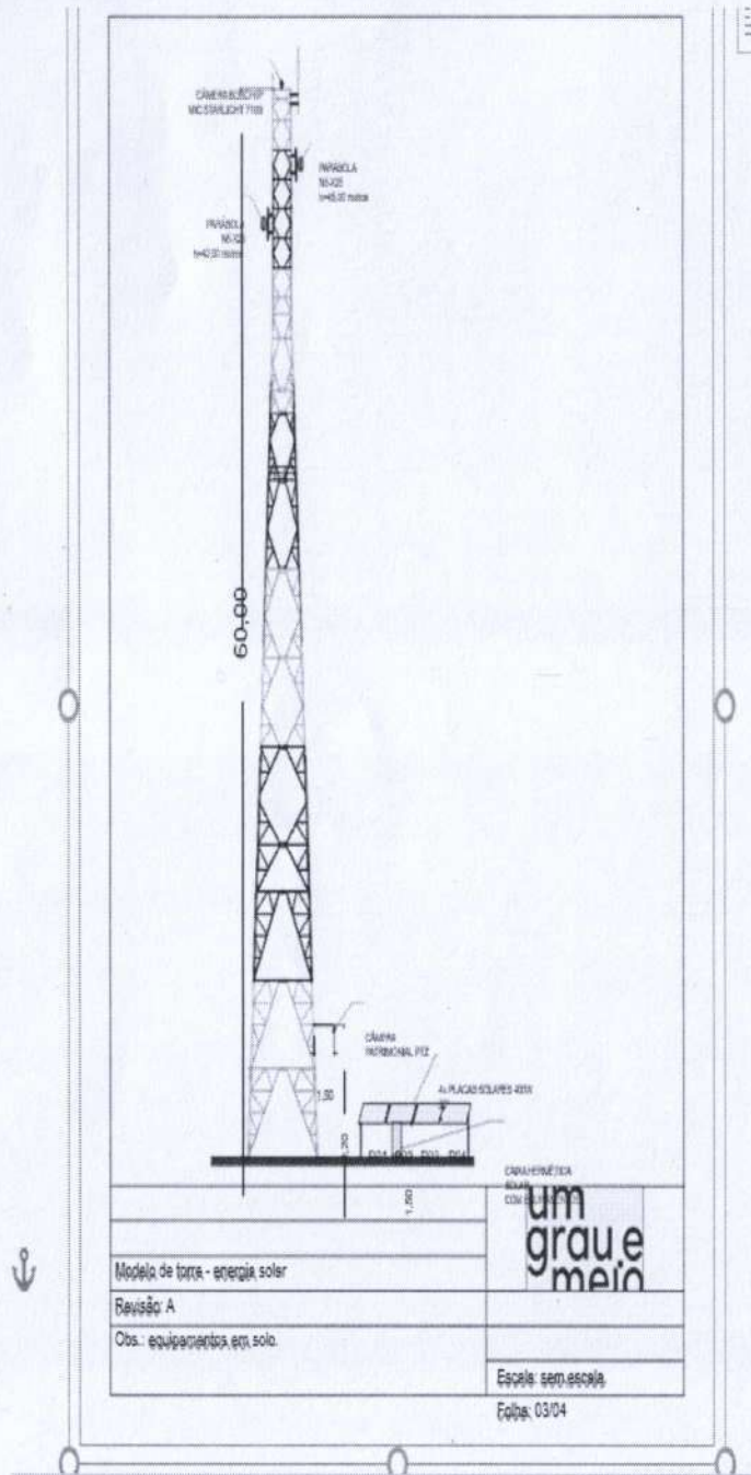
(TowerInfrastructureDetails)
